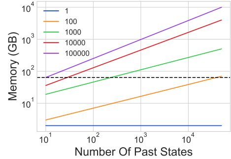
Fig. 8: Memory overheads incurred by RL-S2V as the number of saved past states ( x -axis) and edge additions (line color) increases. The black dashed line denotes the available memory on our test server. RL-S2V can retain a large number of past states for small graph transformations; however, its per-state memory requirements become unwieldy when attempting transformations of the size required to evade Prov-HIDS.
